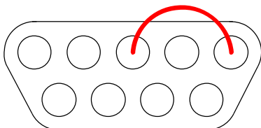
BRAKE 100%
