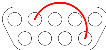
CLUTCH 0%
